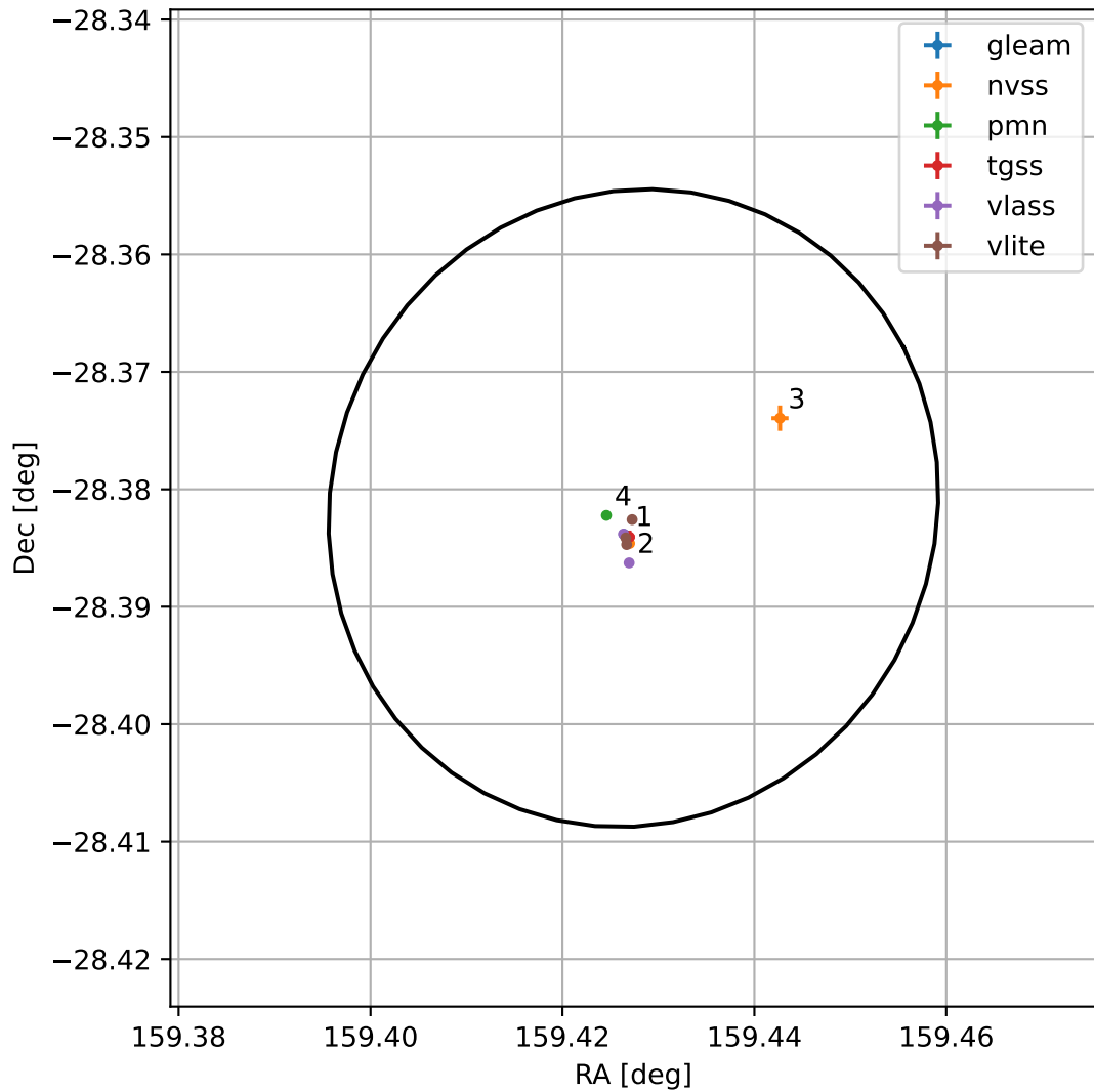
4FGL J1037.7-2822
