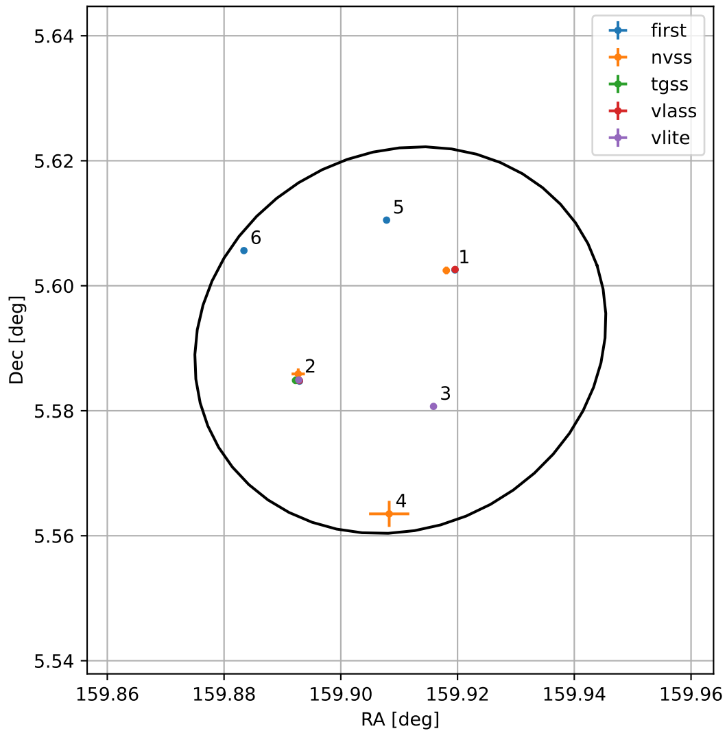
4FGL J1039.6+0535
