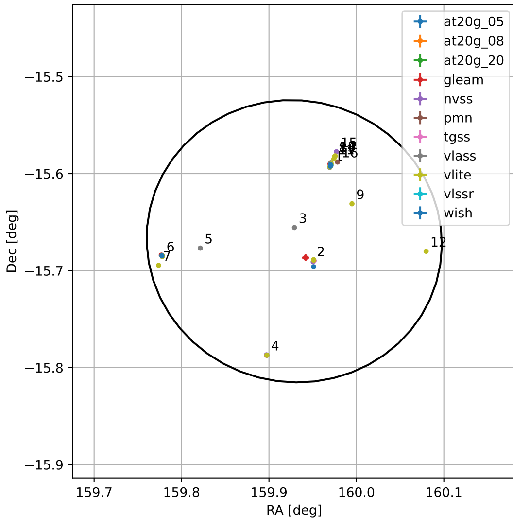
4FGL J1039.7-1540
