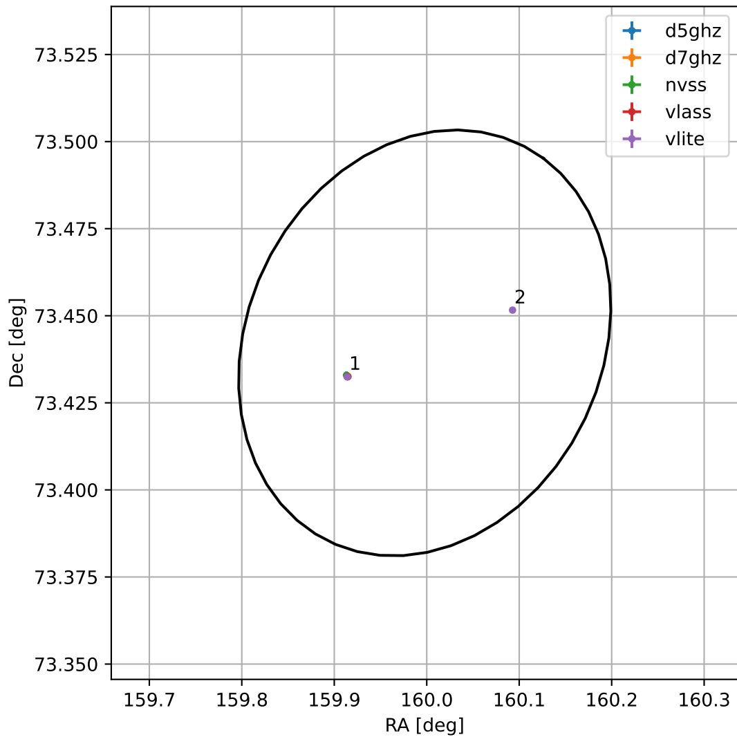
4FGL J1039.9+7326
