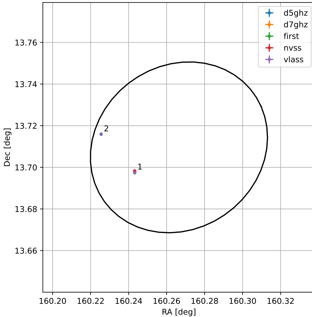
4FGL J1041.0+1342
