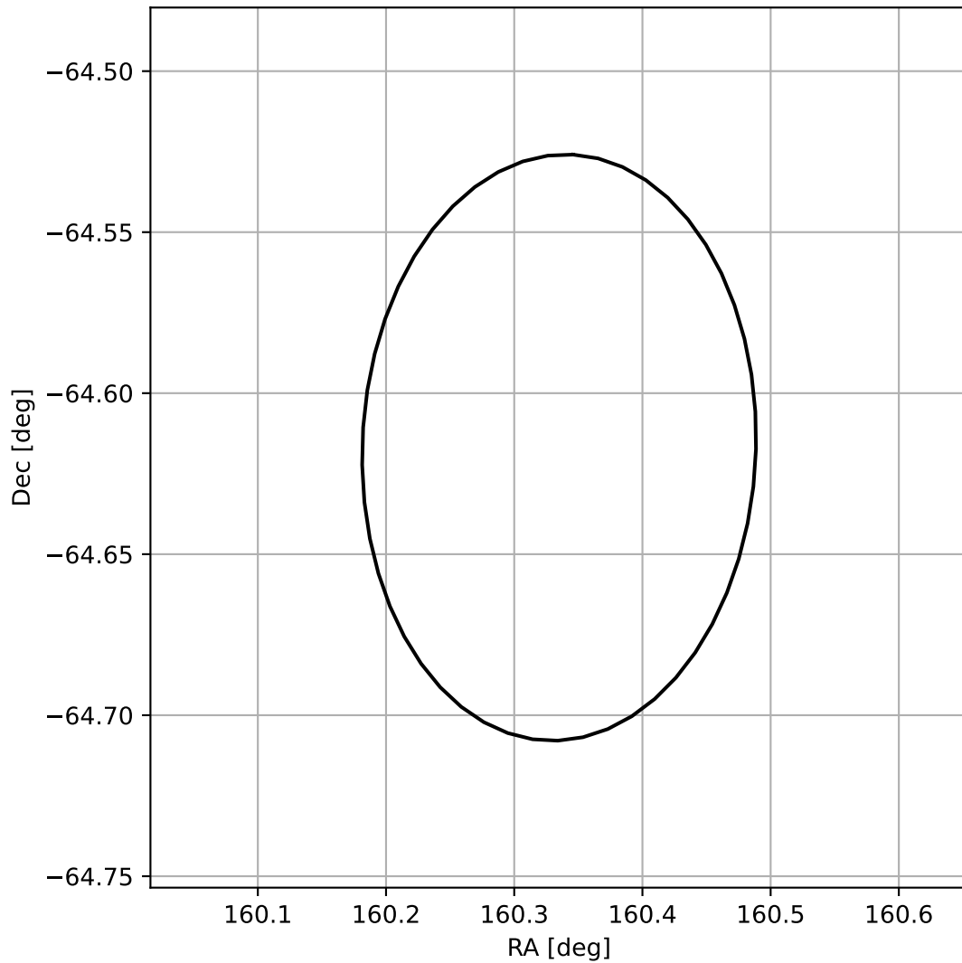
4FGL J1041.3-6437
