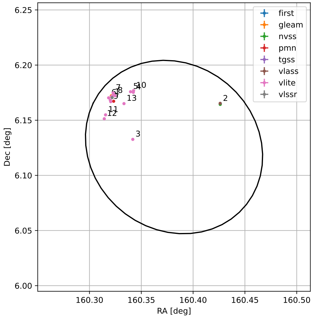
4FGL J1041.5+0607
