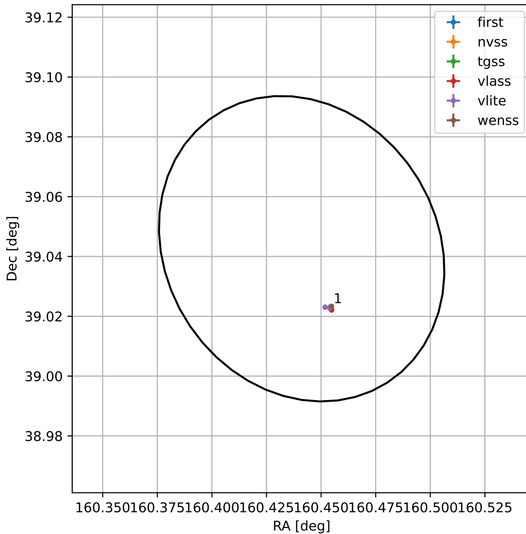
4FGL J1041.7+3902
