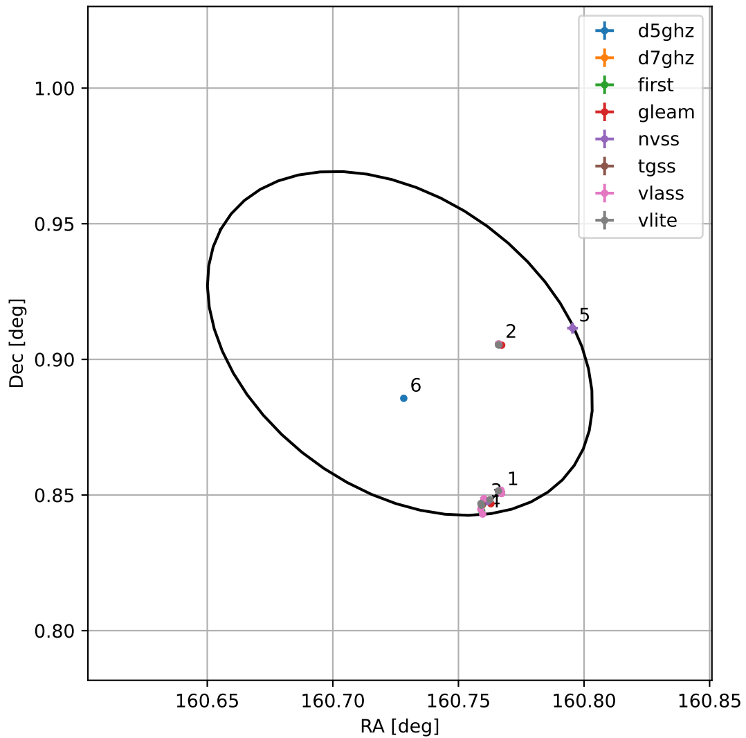
4FGL J1042.9+0054
