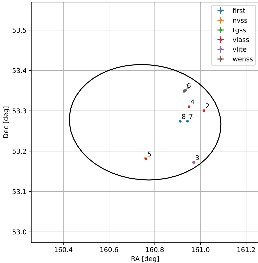
4FGL J1043.0+5316
