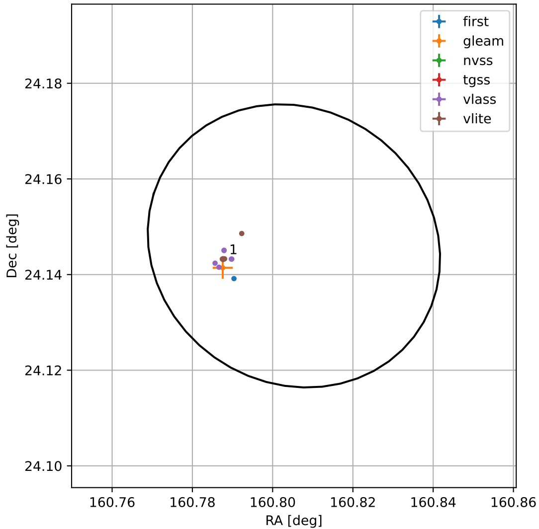
4FGL J1043.2+2408
