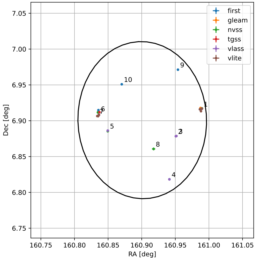
4FGL J1043.6+0654
