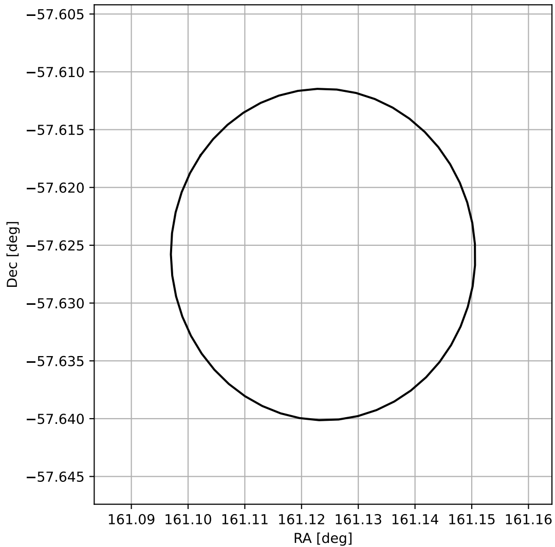
4FGL J1044.4-5737
