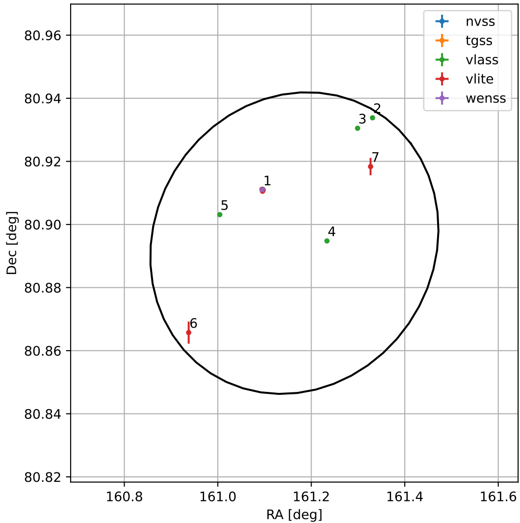
4FGL J1044.6+8053
