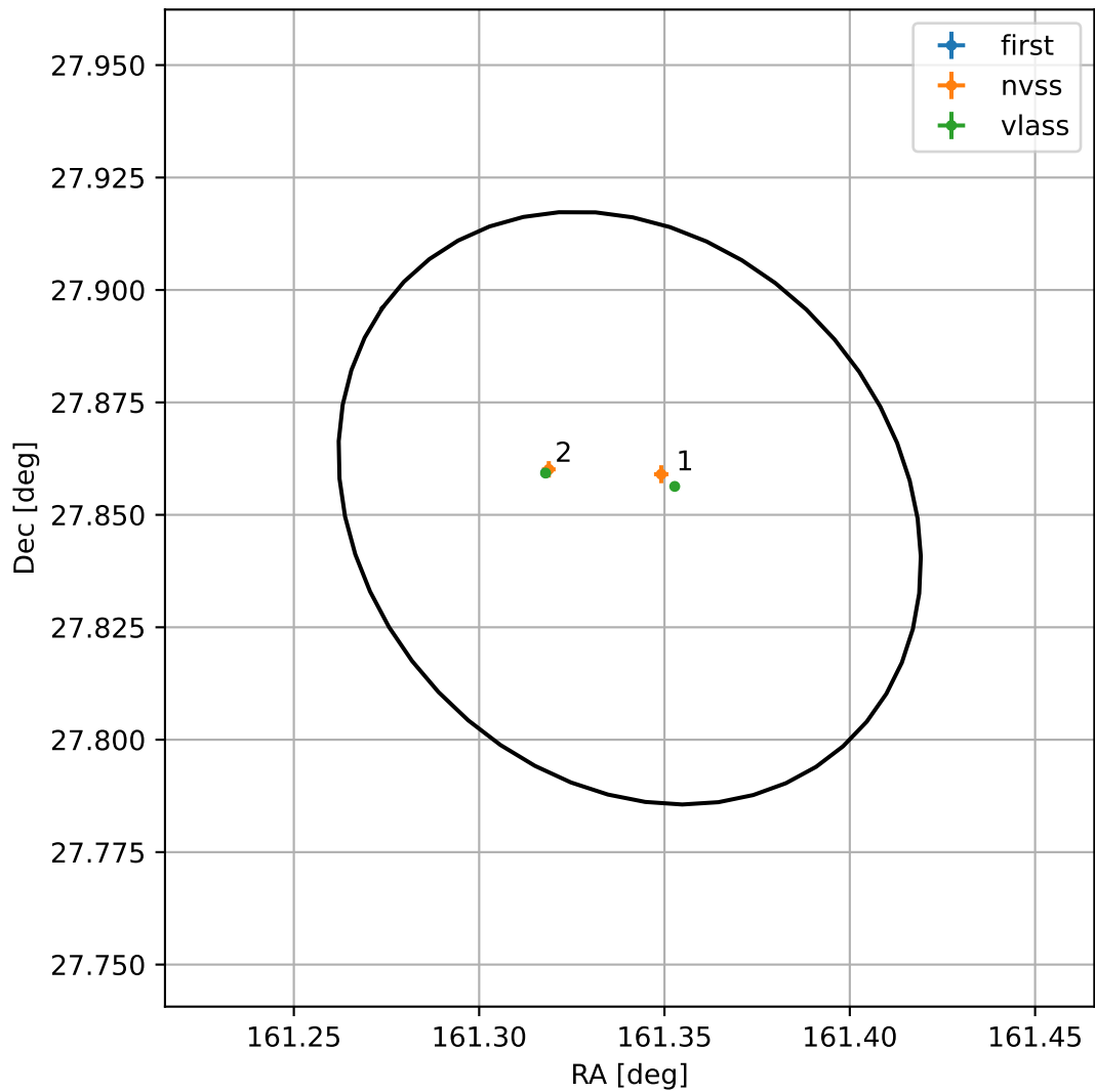
4FGL J1045.3+2751
