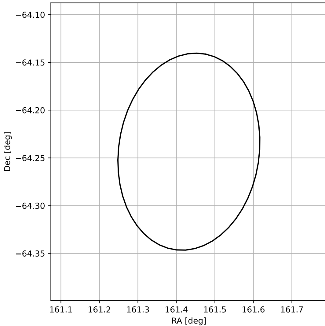
4FGL J1045.7-6414
