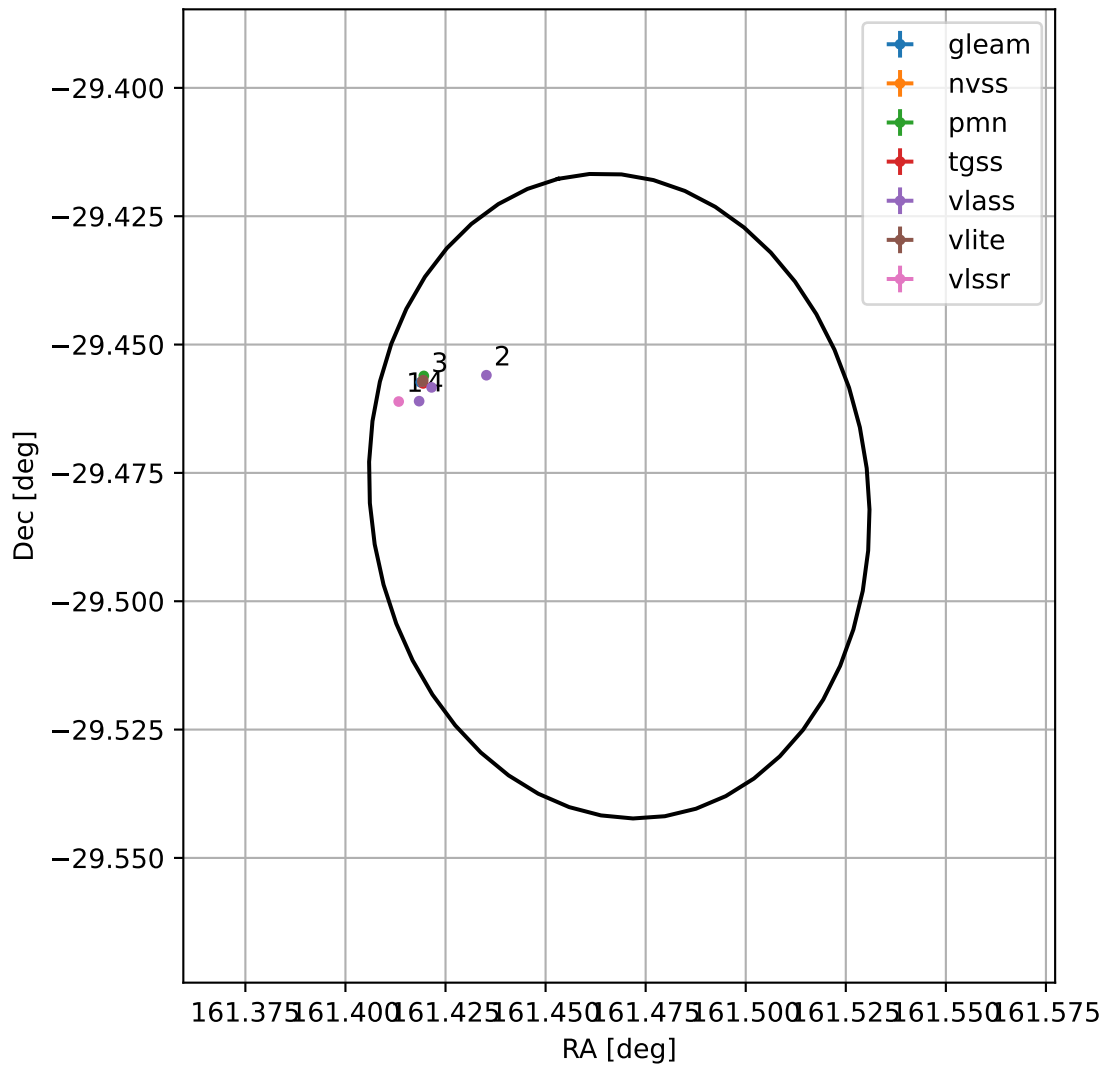
4FGL J1045.8-2928
