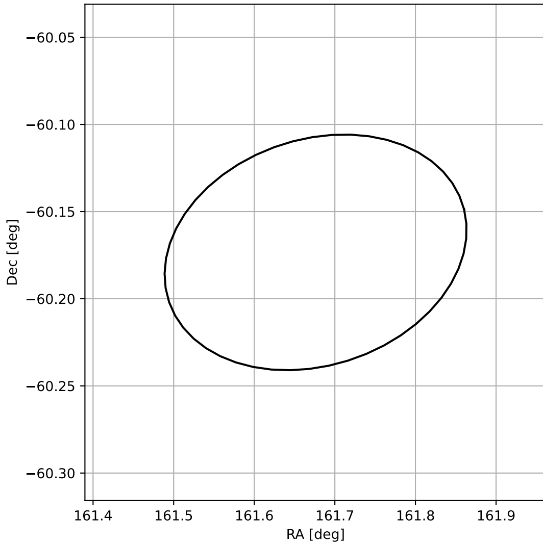
4FGL J1046.7-6010
