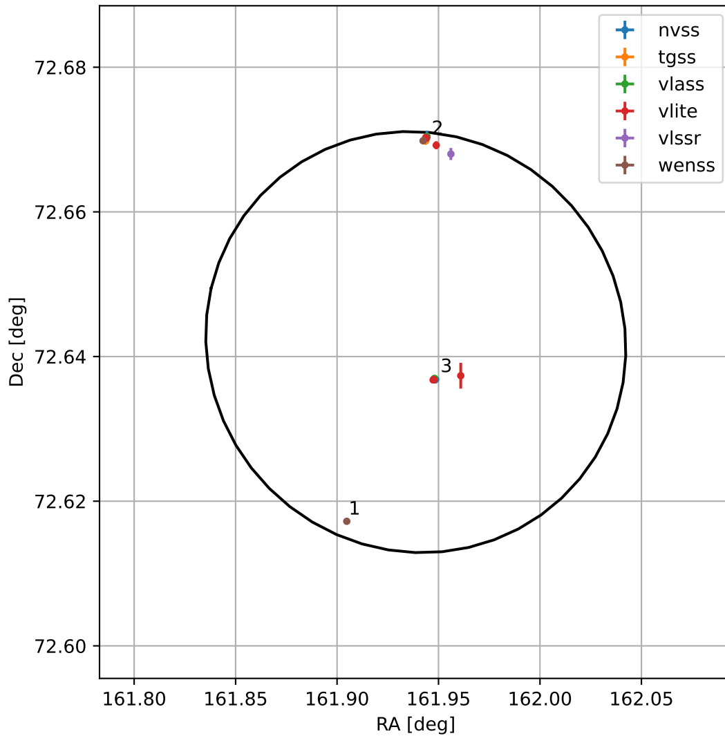
4FGL J1047.7+7238
