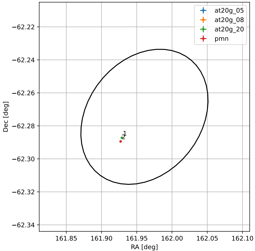
4FGL J1047.8-6216
