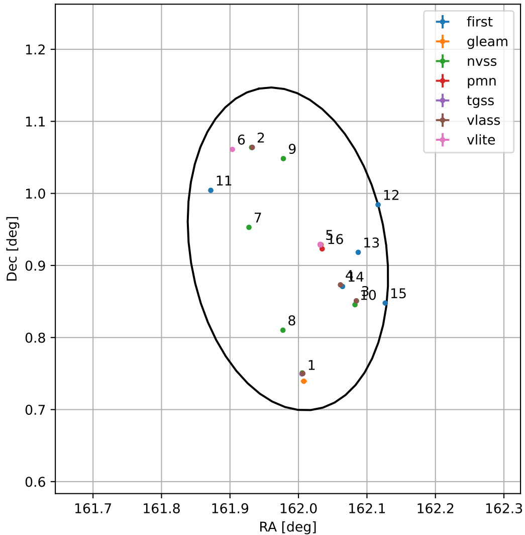
4FGL J1047.9+0055
