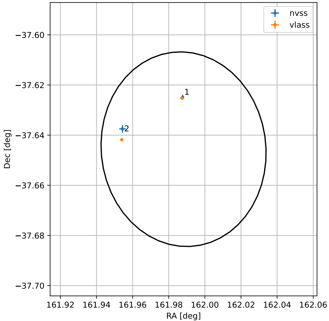
4FGL J1047.9-3738
