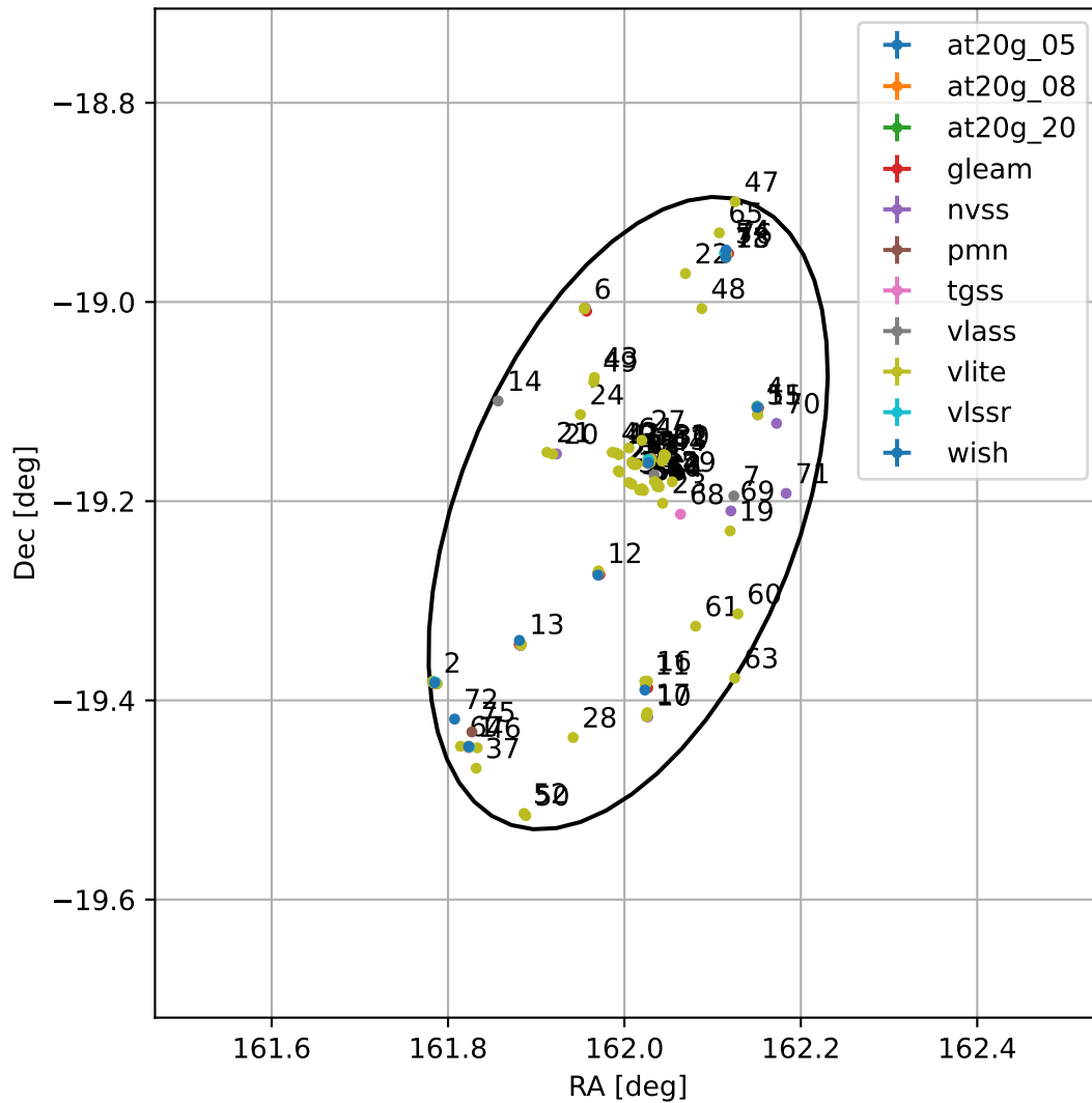
4FGL J1048.0-1912
