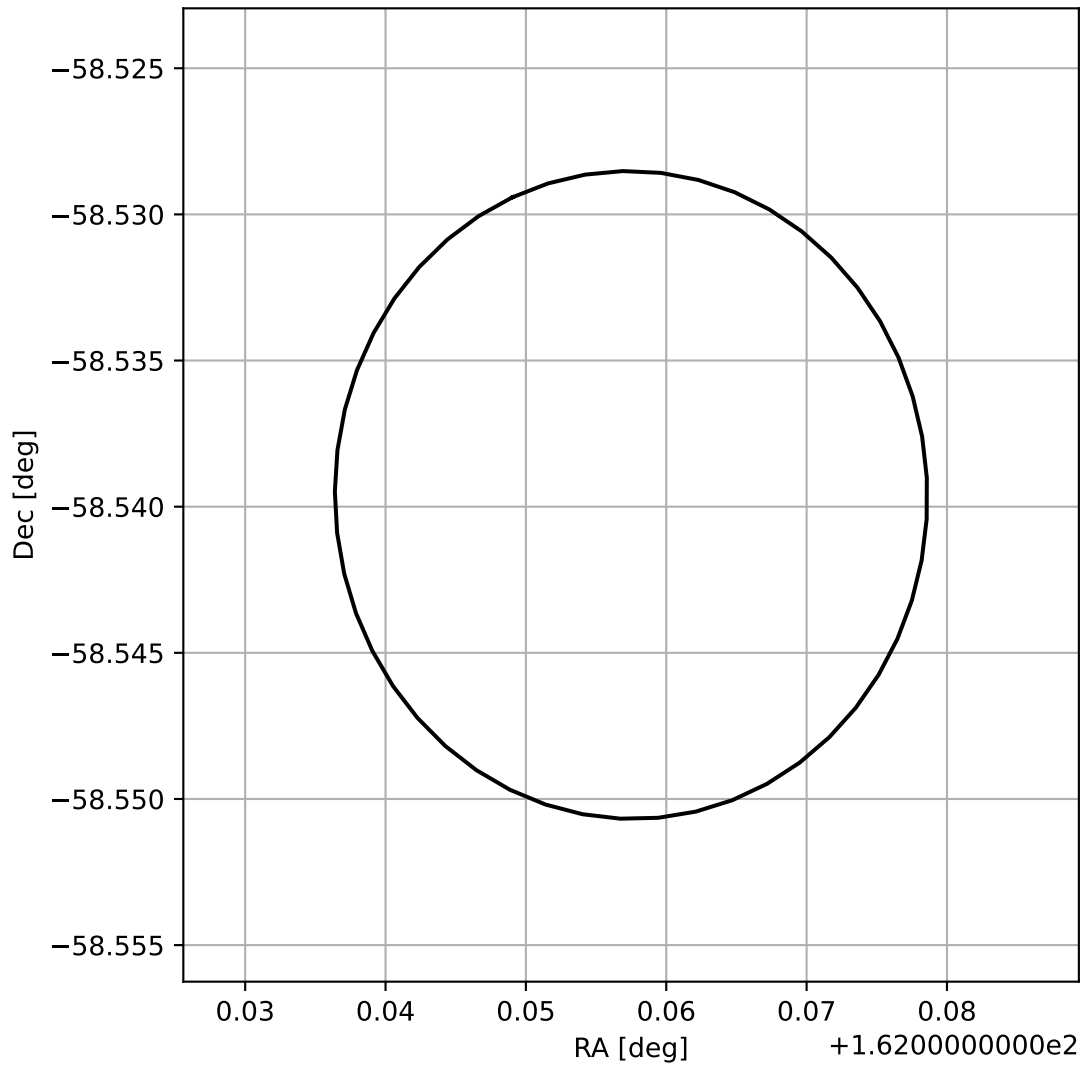
4FGL J1048.2-5832
