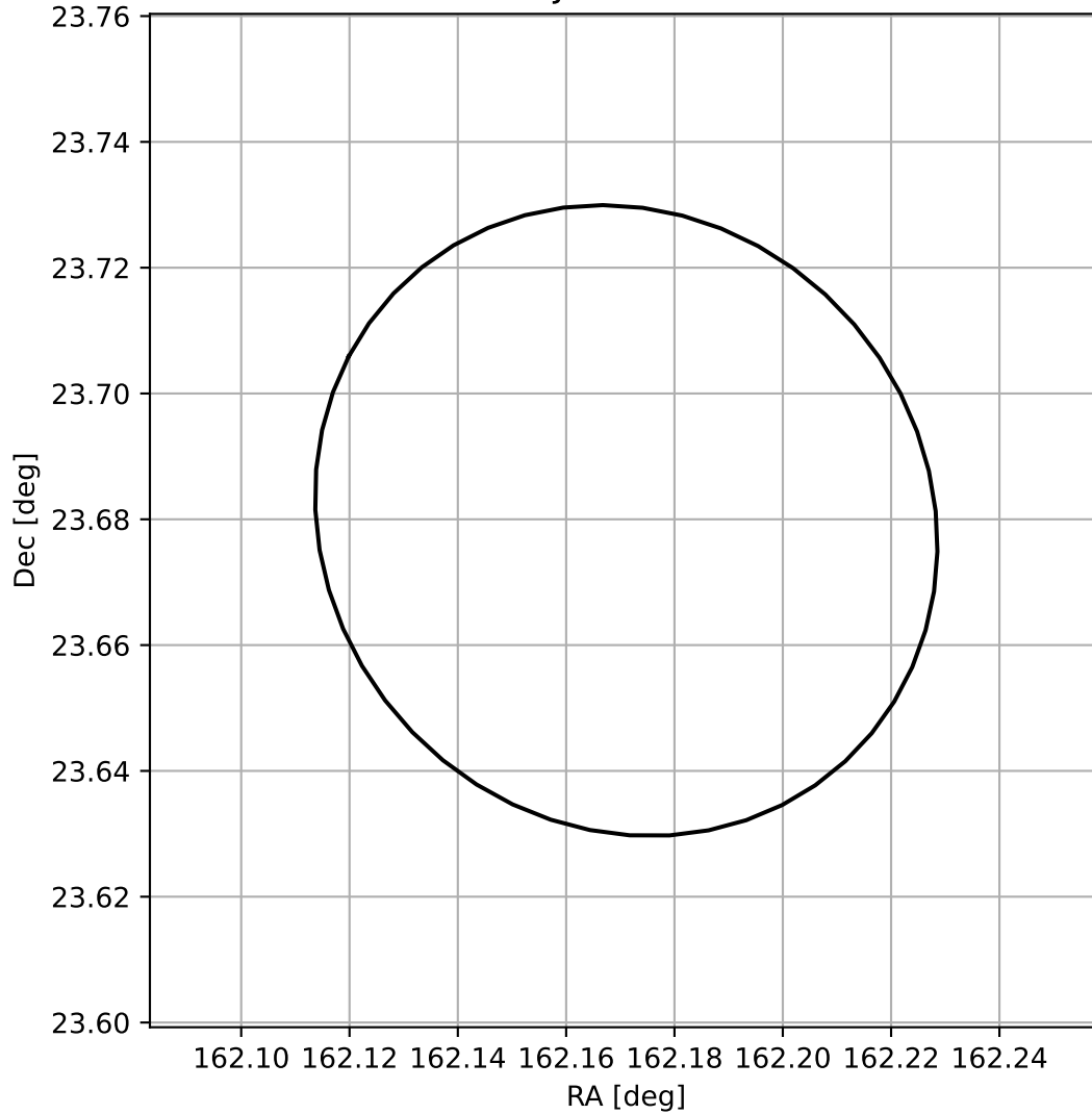
4FGL J1048.6+2340
