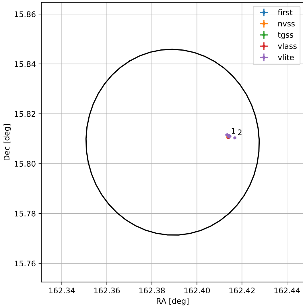
4FGL J1049.5+1548
