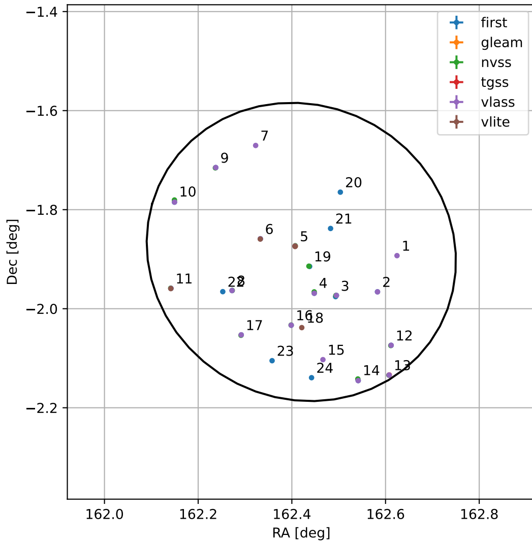
4FGL J1049.6-0153
