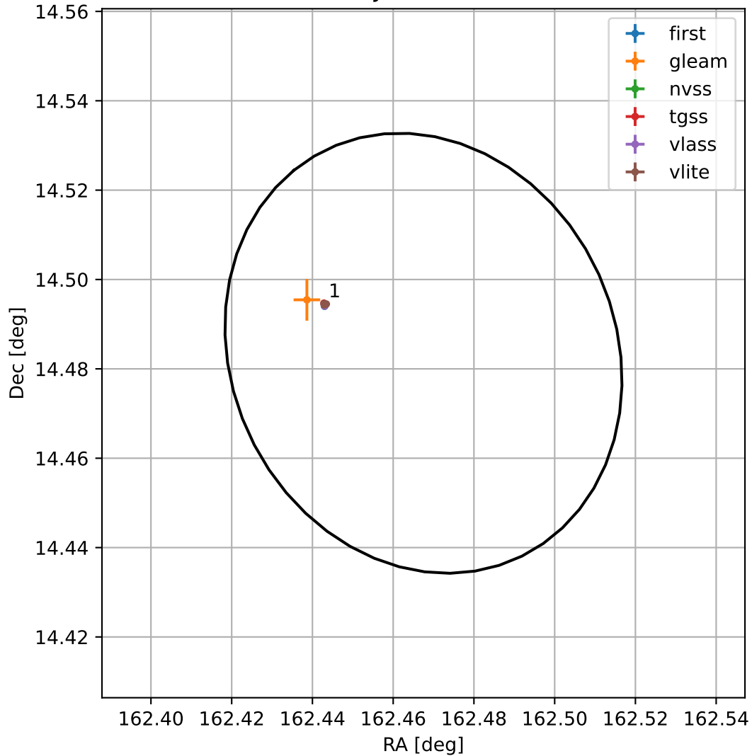
4FGL J1049.8+1429
