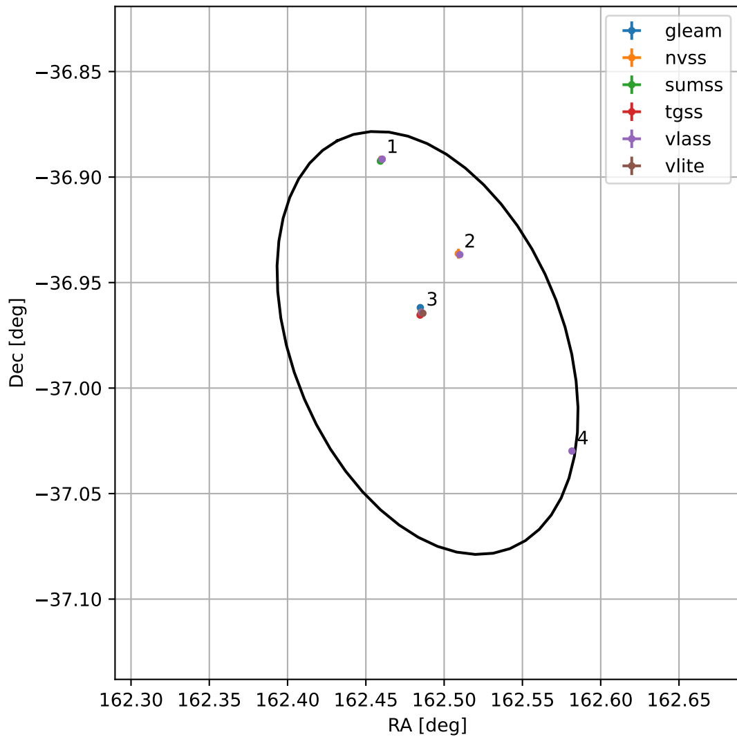
4FGL J1049.9-3658
