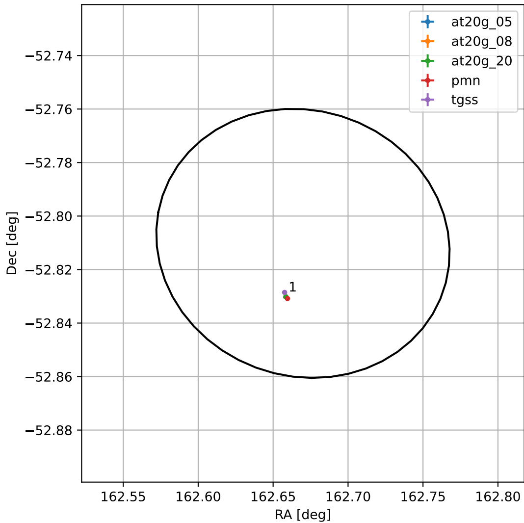
4FGL J1050.6-5248
