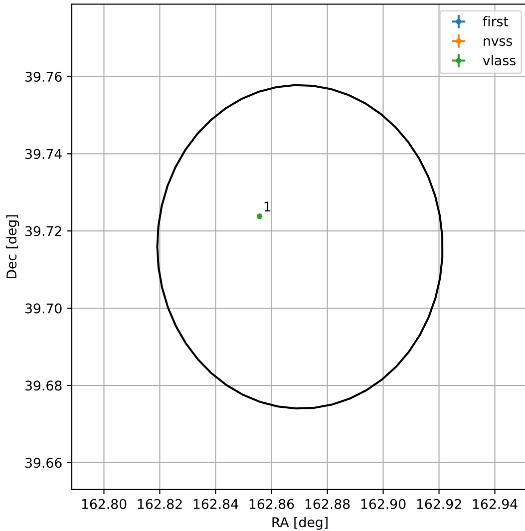
4FGL J1051.4+3942
