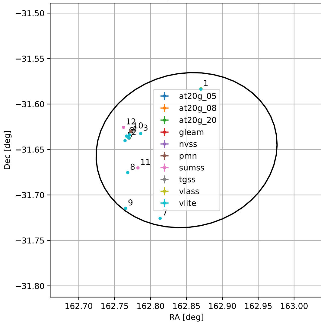
4FGL J1051.4-3139
