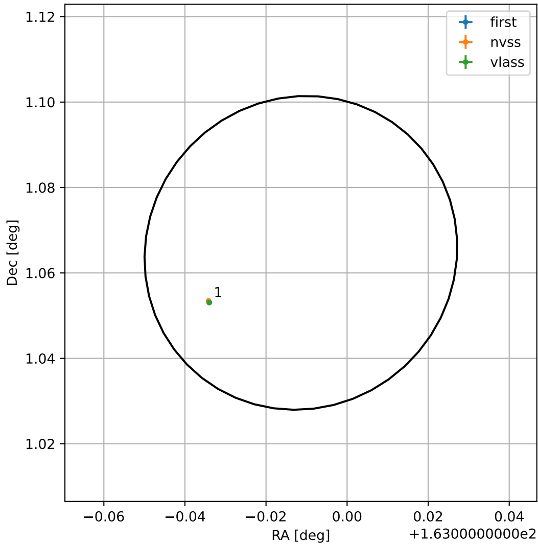
4FGL J1051.9+0103
