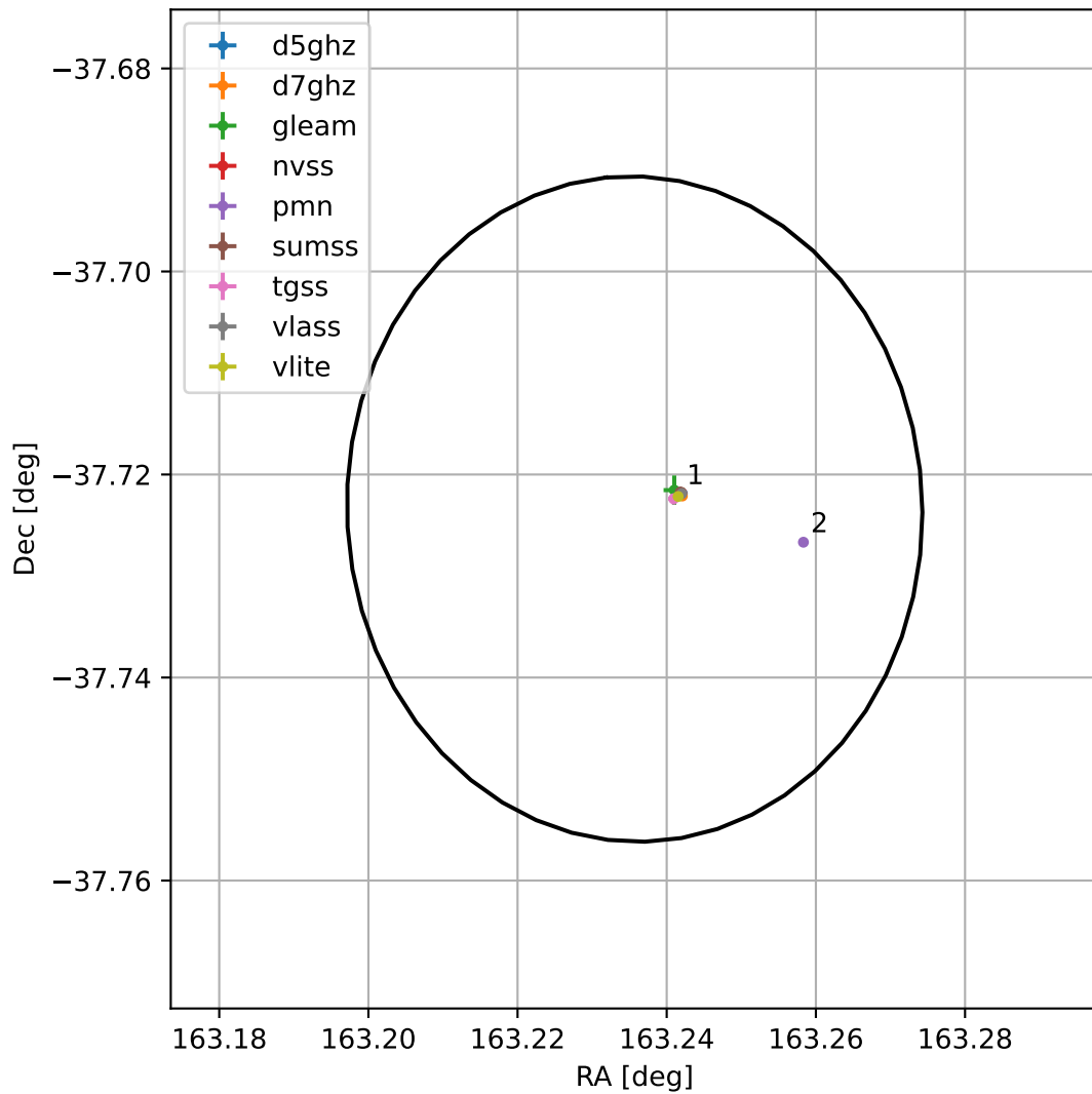
4FGL J1052.9-3743
