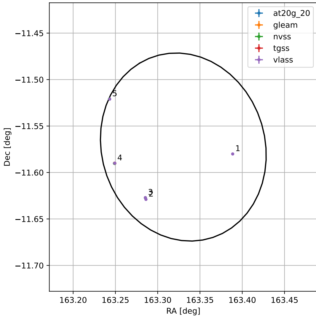
4FGL J1053.3-1134
