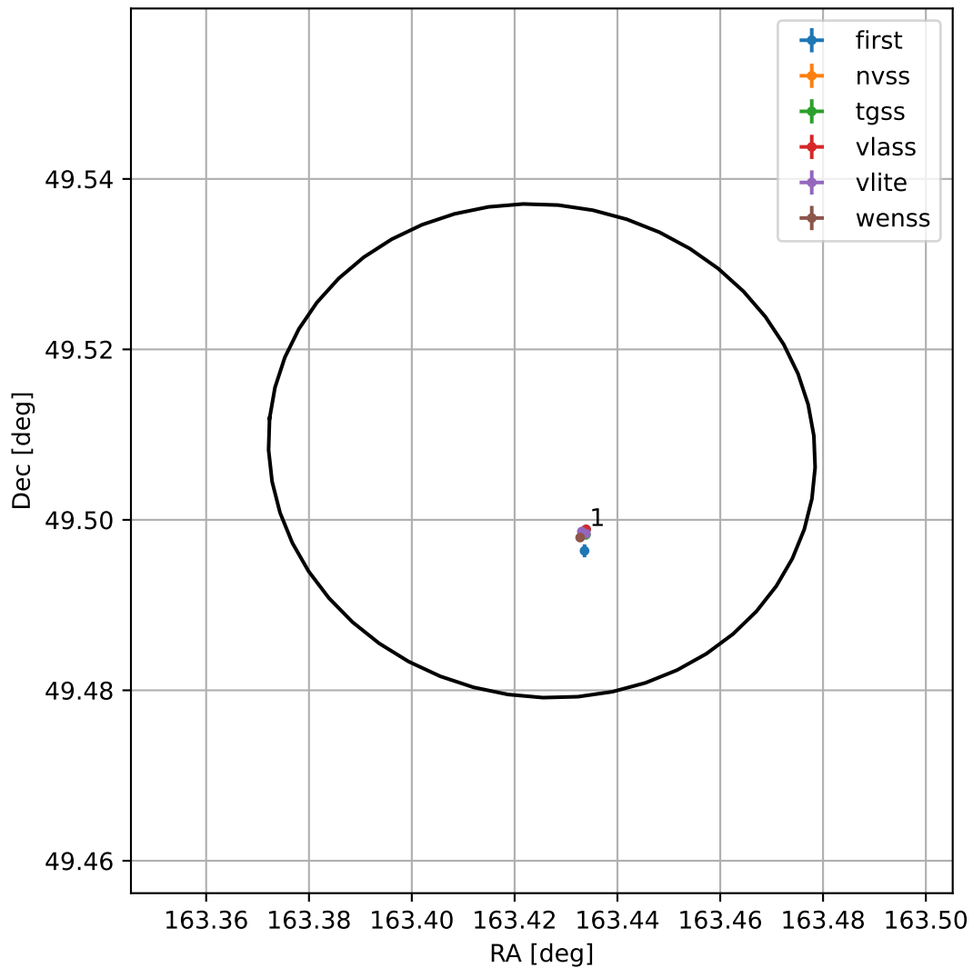
4FGL J1053.7+4930
