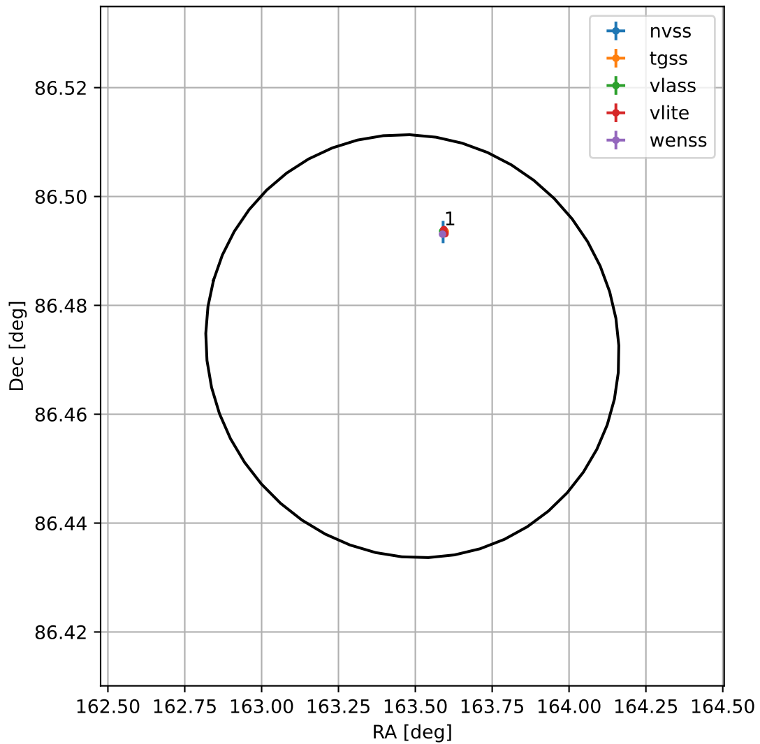
4FGL J1053.9+8628
