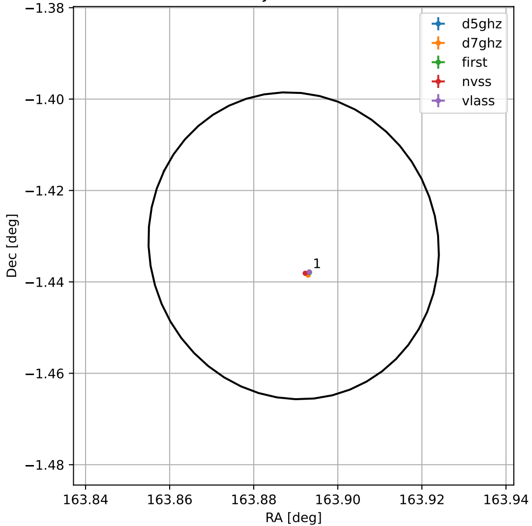
4FGL J1055.5-0125
