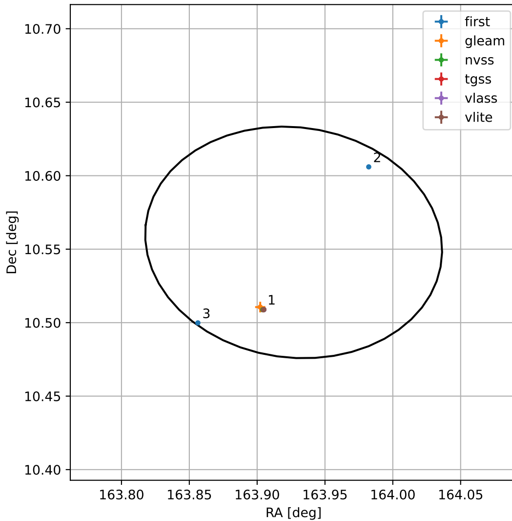
4FGL J1055.7+1033
