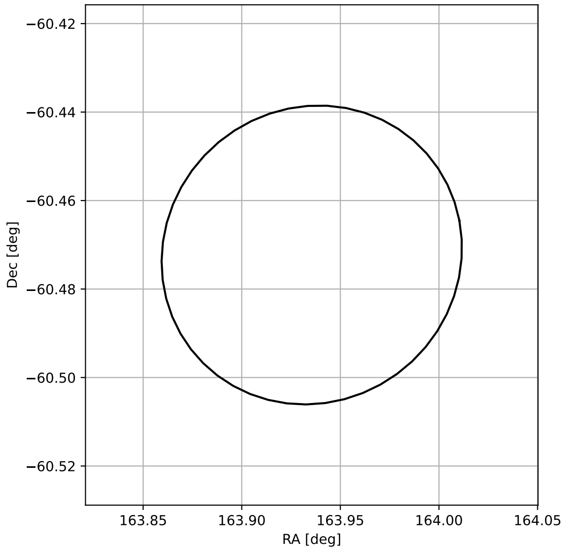
4FGL J1055.7-6028
