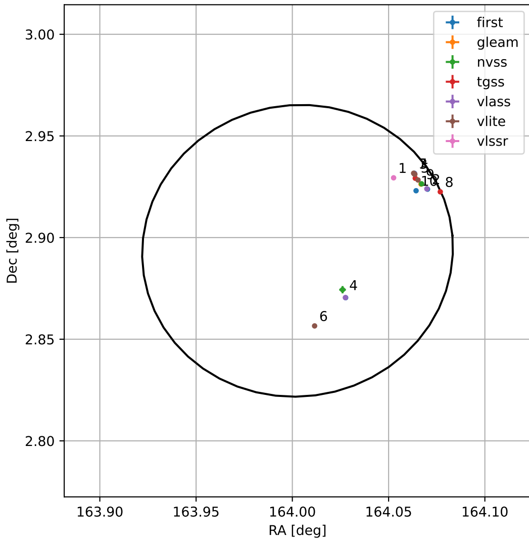
4FGL J1056.0+0253
