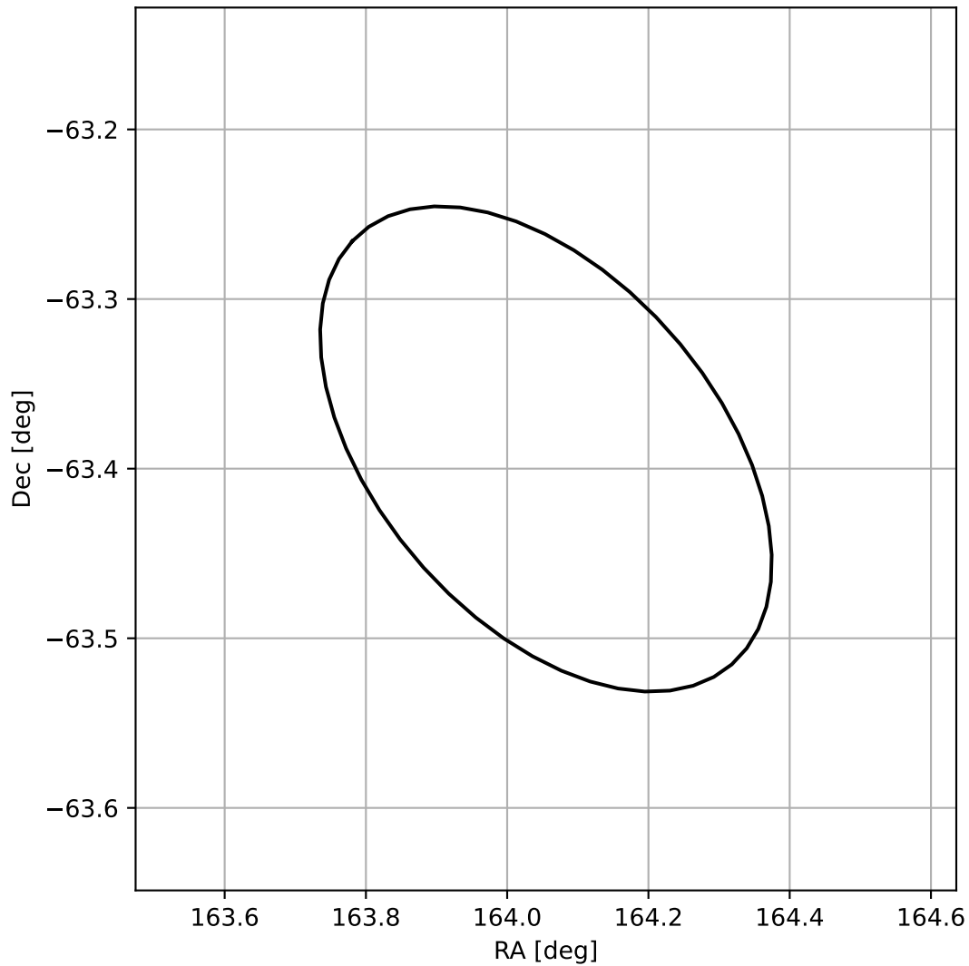
4FGL J1056.2-6323
