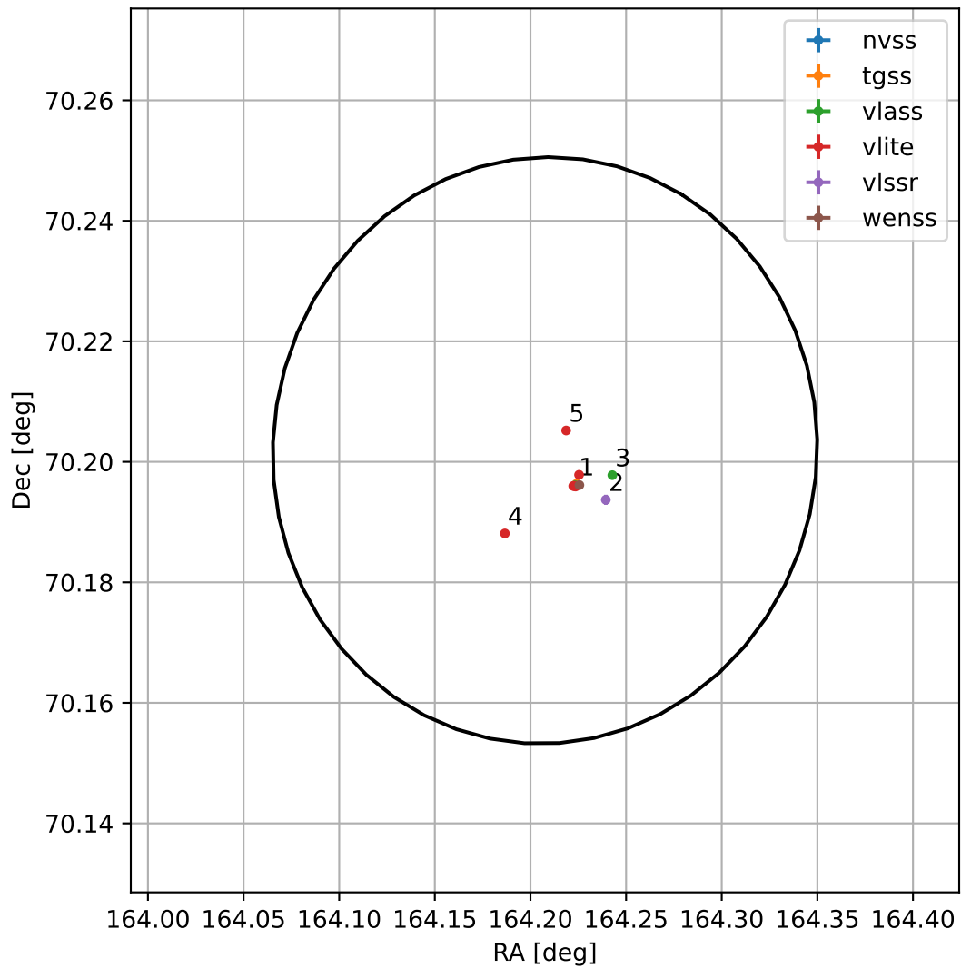
4FGL J1056.8+7012
