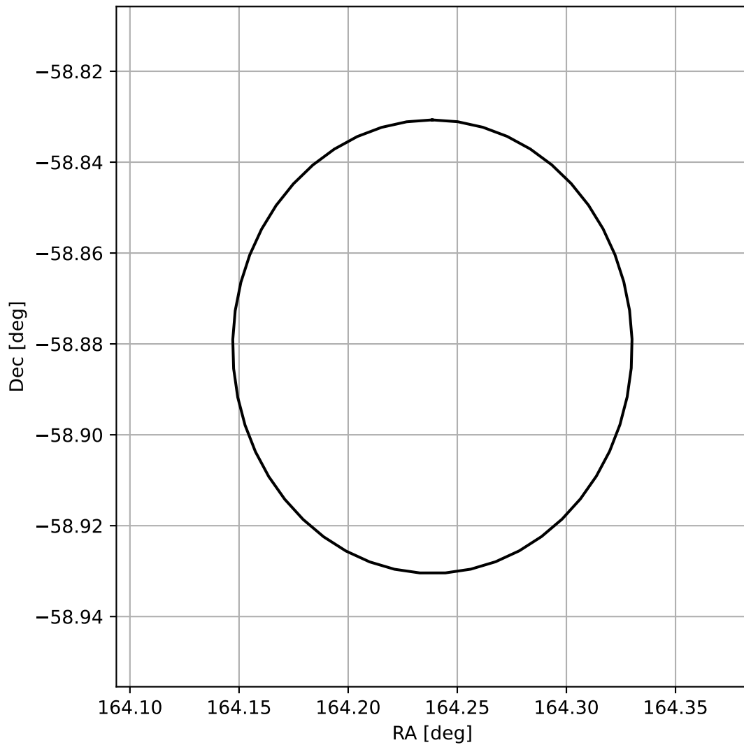
4FGL J1056.9-5852
