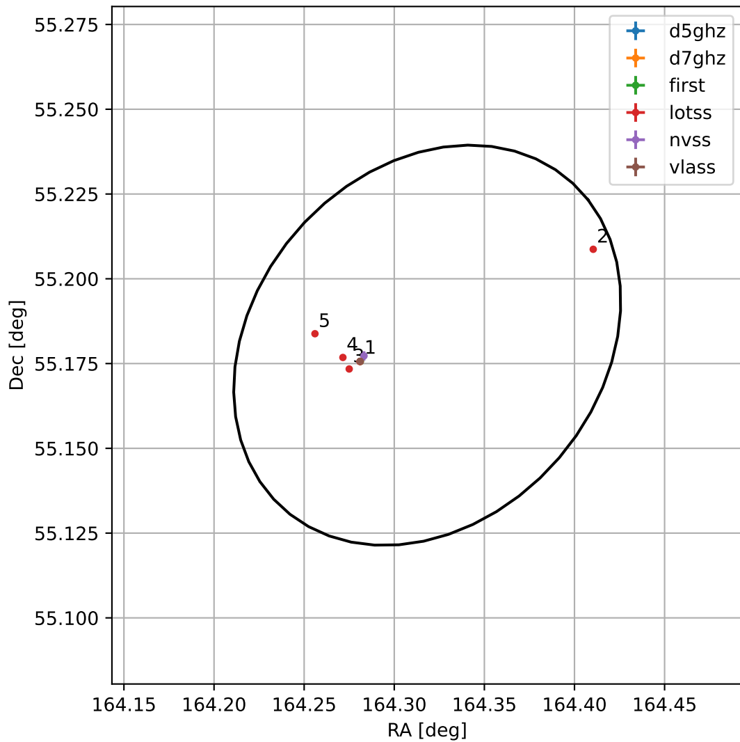
4FGL J1057.2+5510
