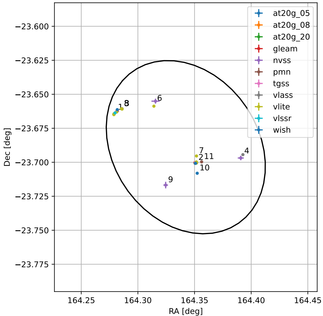
4FGL J1057.3-2341
