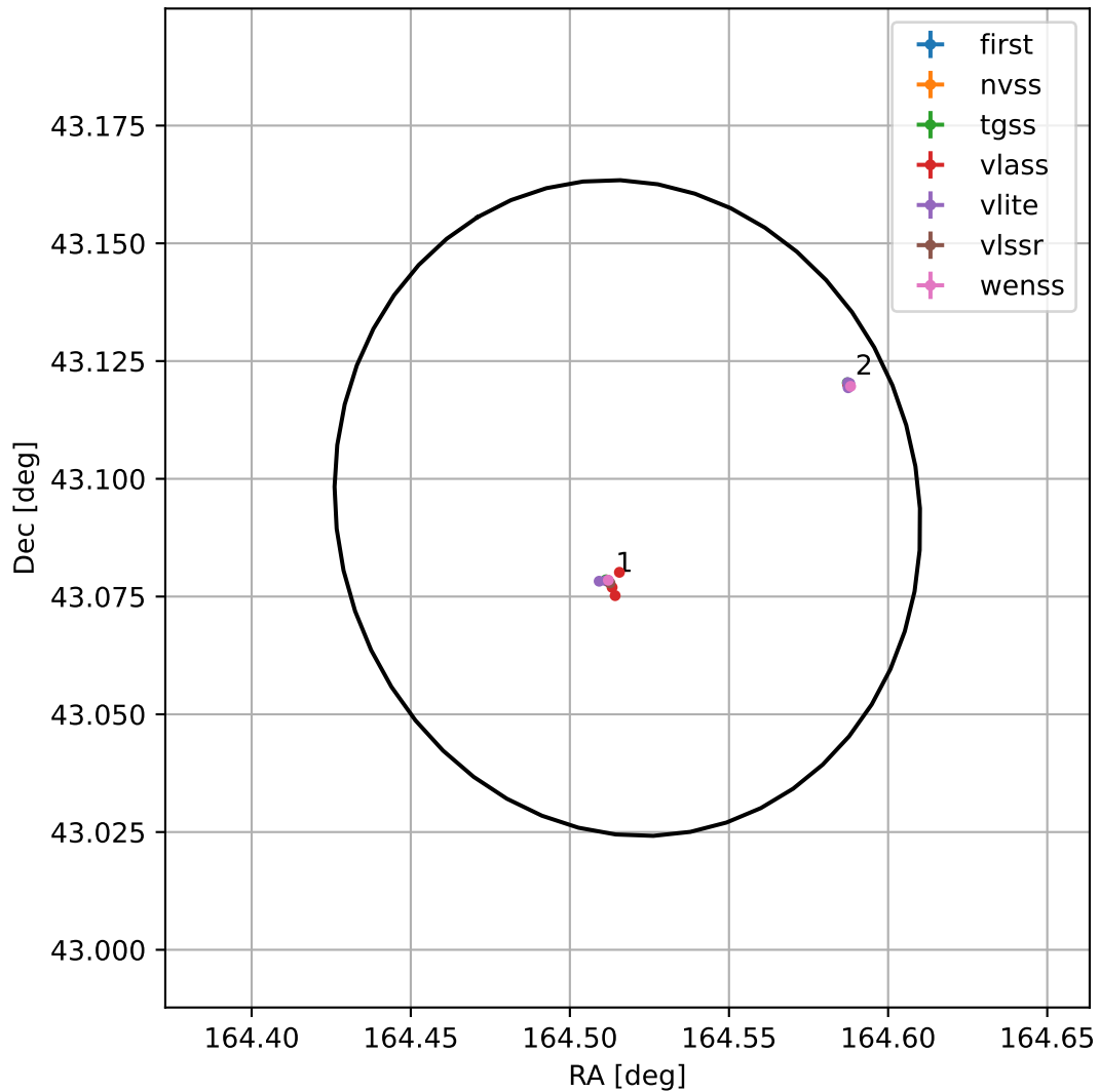
4FGL J1058.0+4305
