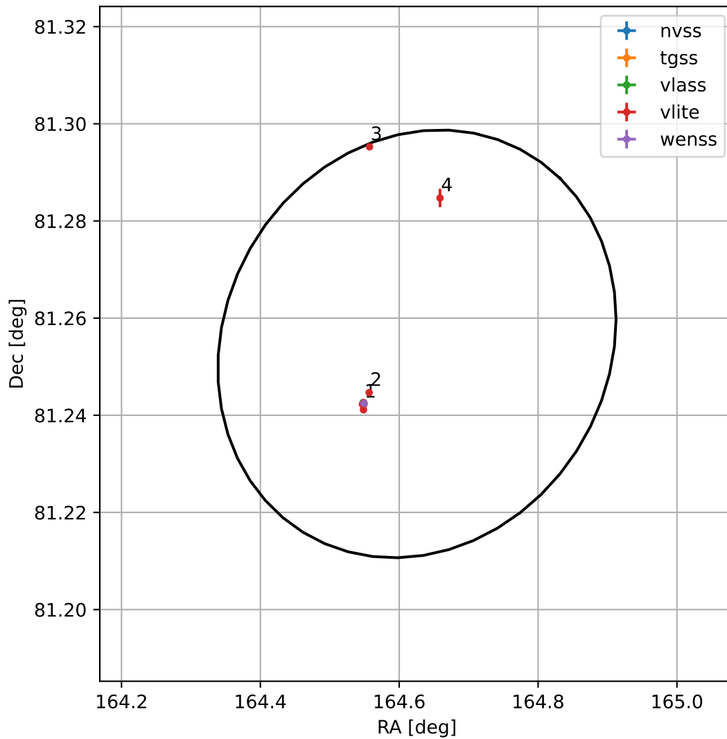
4FGL J1058.5+8115
