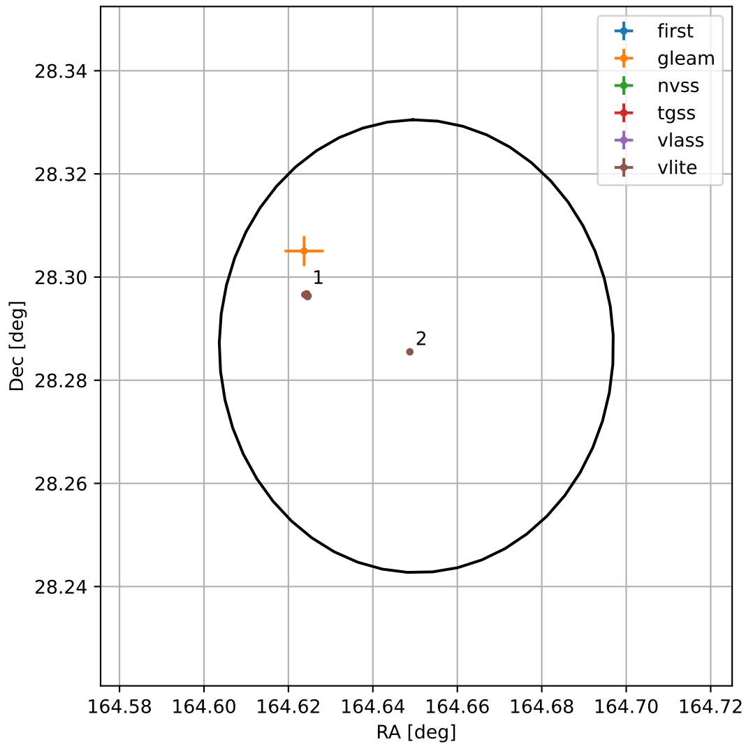
4FGL J1058.6+2817
