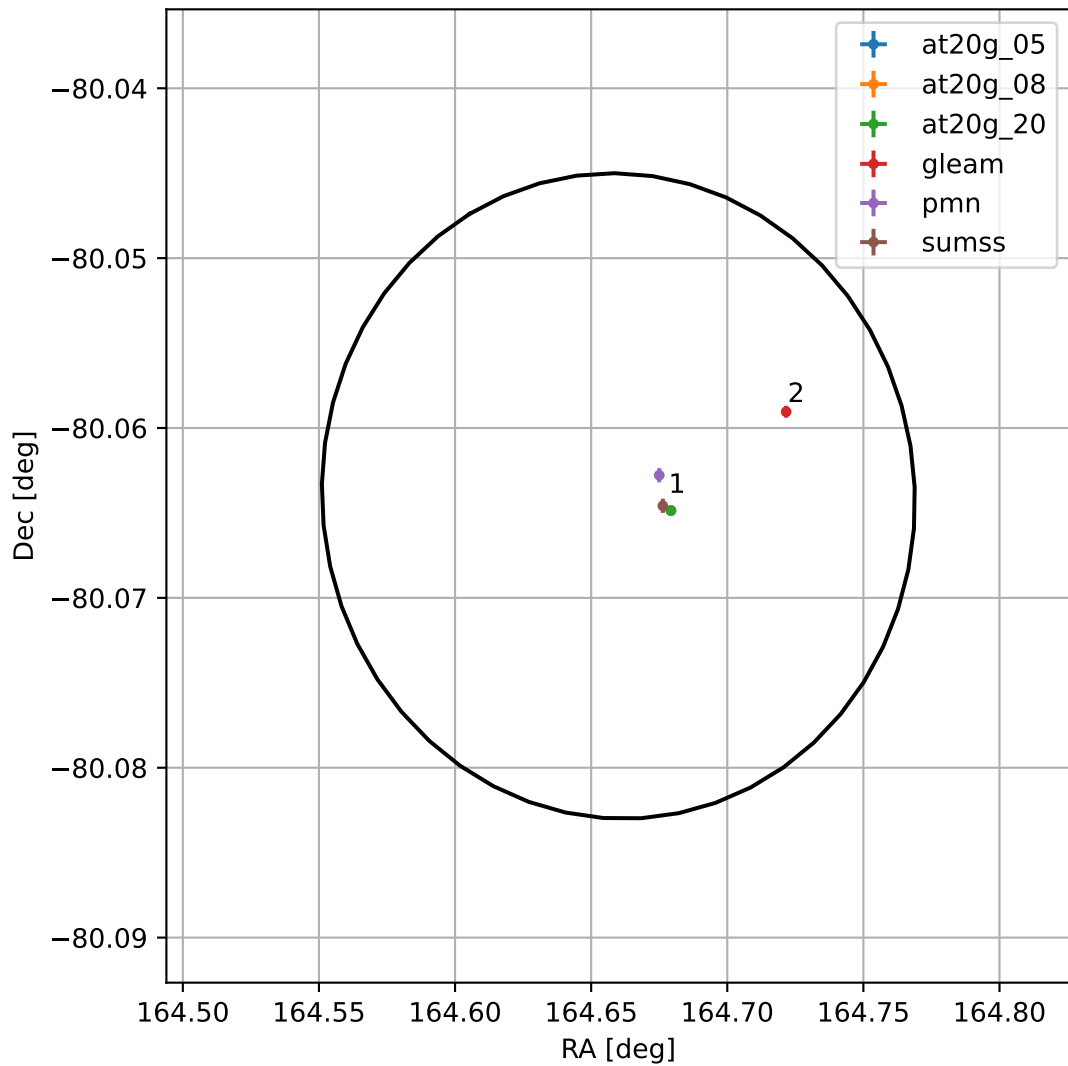
4FGL J1058.6-8003
